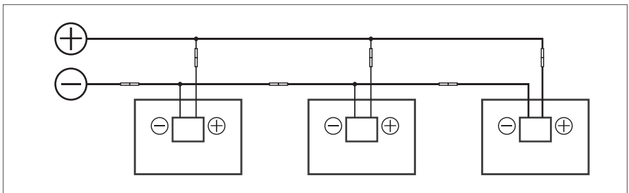
(Figure 10: Parallel connection diagram)
