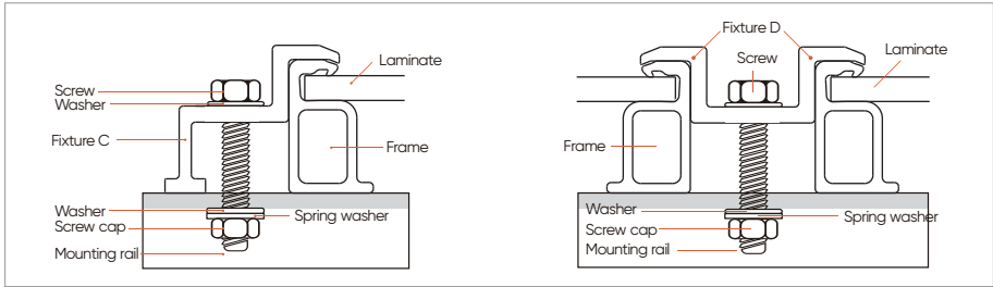
(Figure 6: Hybrid frame module Fixture Installation Diagram)
