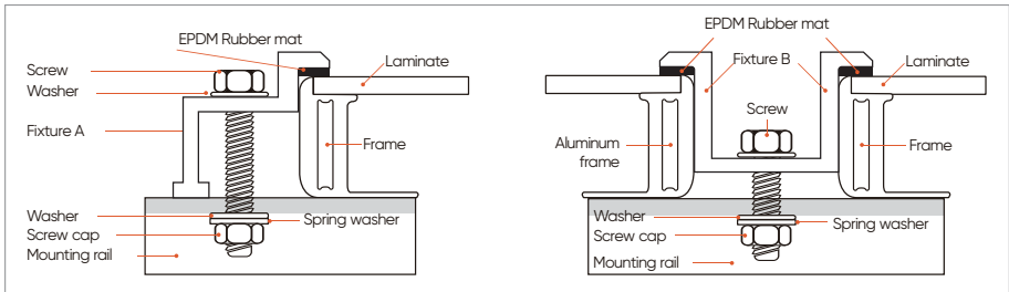
(Figure 7: Full-Screen PV Module Fixture Installation Diagram)
