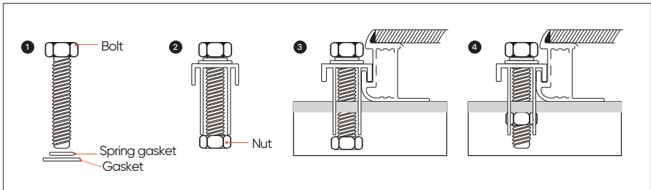
(Figure 8 Installation Detail with Side Fixture)
