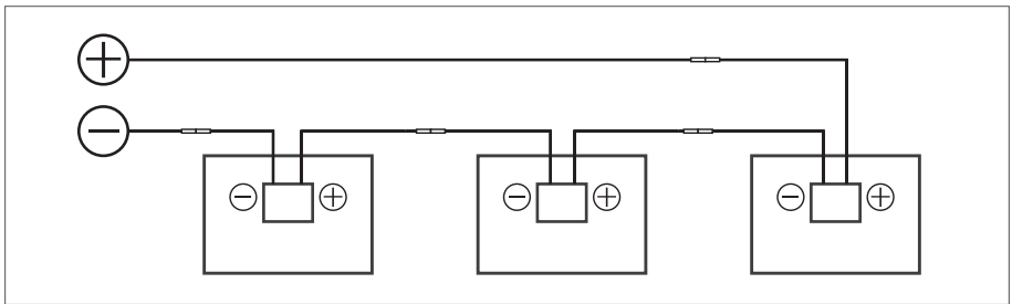
(Figure 9: Series connection diagram)
