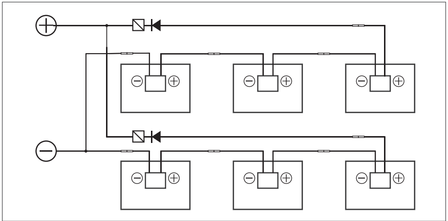
(Figure 11: Series-parallel connection diagram)
