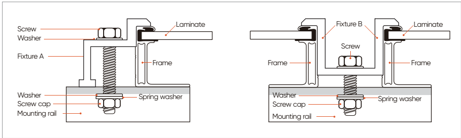
(Figure 5: Regular PV Module Fixture Installation Diagram)
