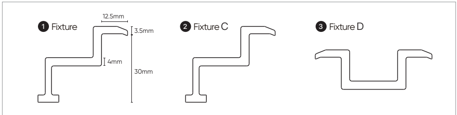
Figure 3: Fixture Diagram of hybrid frame PV Module
