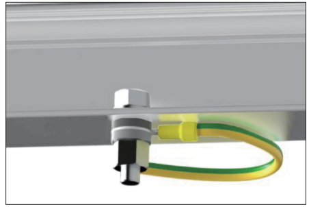
(Figure 13: Schematic diagram of bolt grounding)
