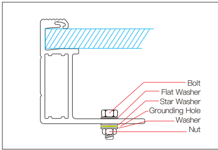
(Figure 13: Schematic diagram of bolt grounding)
