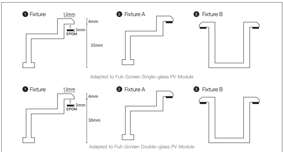
(Figure 4: Fixture Diagram of Full-Screen PV Module)
